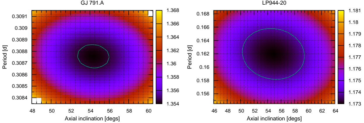
Fig. 2.— Reduced \chi^2 ( \chi_r^2 ) plots of rotation period, P , vs axial inclination, i with 67.3% confidence level. \chi_{r,\min}^2 = 1.354 (GJ 791.2A) and \chi_{r,\min}^2 = 1.173 (LP 944-20). The derived parameters and uncertainties are listed in Table 1.
