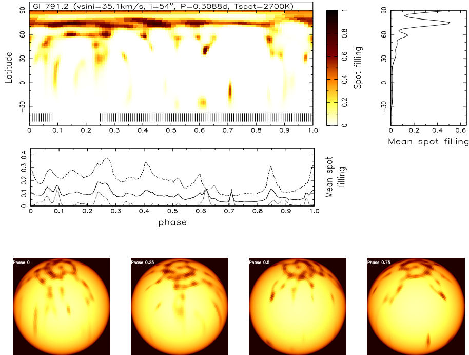
Fig. 6.— Maximum entropy regularized image reconstructions of GJ 791.2A plotted as Mercator (top) and 3D projections (bottom). The image of GJ 791.2A is shown for parameters optimised with T_{\text{phot}} = 3000 K and T_{\text{spot}} = 2700 K, which have a contrast ratio at disk center of I_{\text{spot}}(0)/I_{\text{phot}}(0) = 0.41 . The tick marks in the Mercator plot indicate the phases of observation. The latitudinal mean spot filling is shown in the upper left panel. The mean phase spot filling is indicated in the panel below the Mercator map for latitudes -30^\circ to 90^\circ (solid line), -30^\circ to 45^\circ (dotted line) and 45^\circ to 90^\circ (dashed line).
