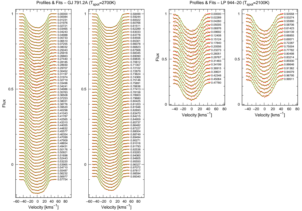
Fig. 3.— Deconvolved profiles for GJ 791.2A (left) and LP 944-20 (right). The data are plotted as points along with the error bars. The maximum entropy regularised profiles corresponding to the images in Figures 6 & 8 are shown as line plots. Observations are phased with epochs \text{HJD0} = 2456904.63601 (GJ 791.2A) and \text{HJD0} = 2456907.73034 (LP 944-20), which are the mid-exposures of the first observation in each time series.
