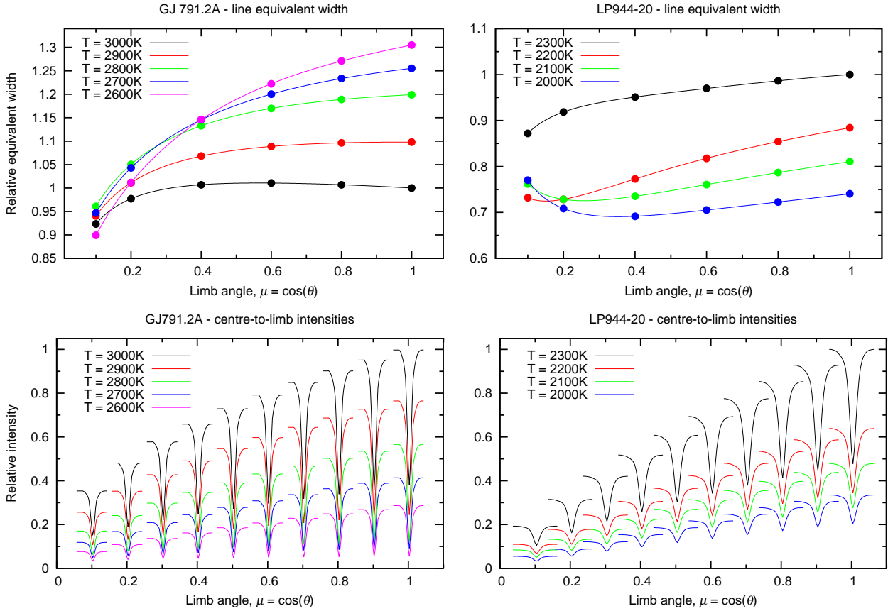
Fig. 1.— Top: The deconvolved equivalent width as a function of limb-angle, \mu , for BT Settl spectra compute with the WITA code (see §3.3 for details). For GJ 791.2A (left), all spectra were deconvolved using a line list with T = 3000 K and for LP 944-20 (right), using a line list with T = 2300 K. Bottom: The center-to-limb local intensity profiles obtained from deconvolved synthetic spectra. The line profiles are derived from our standard stars, GJ105 (M4.5V) and LP888-18 (M7.5V). The center-to-limb variation of profile equivalent width in the upper panels is adopted. The intensities at each limb-angle, obtained from the synthetic spectra, are the mean intensities determined over the appropriate deconvolution wavelength ranges for our target stars.
