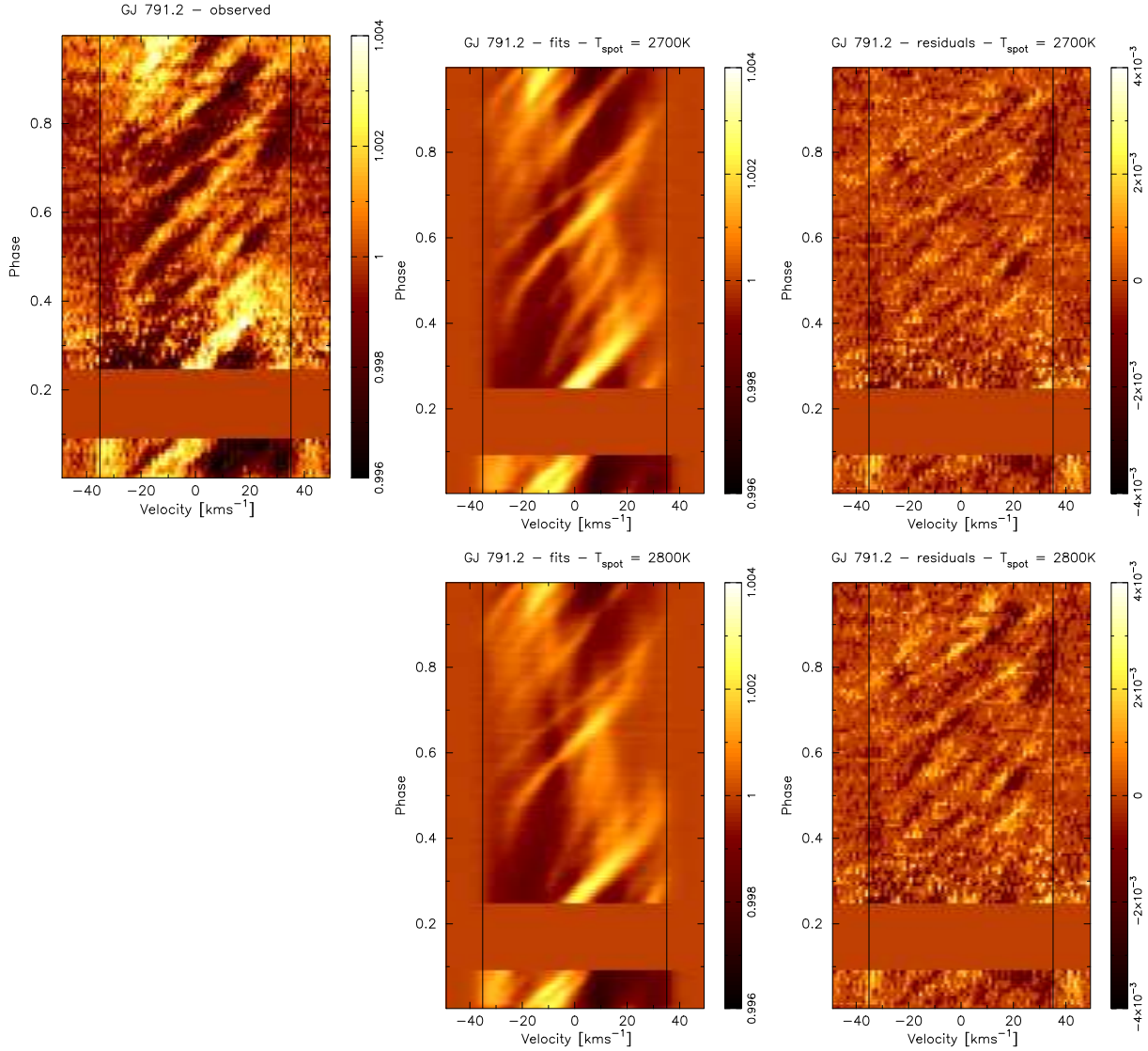
Fig. 4.— Mean profile divided deconvolved line profile time series (left), fits (middle) and fit residuals (right) for GJ 791.2A using a spot temperature of T_{\text{spot}} = 2700\text{K} (upper panels) and T_{\text{spot}} = 2800\text{K} (lower panels). The starspot features appear as white trails while black trails are regions that are more negative relative to the mean profile. The spectra are centered on the observed rest frame and phased according to the adopted 0.3088 d period of GJ 791.2A. The vertical lines indicate a v \sin i profile width of of 35.1 \text{ km s}^{-1} .
