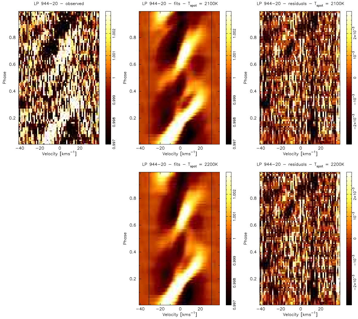
Fig. 5.— As for Figure 4, but for LP 944-20.
