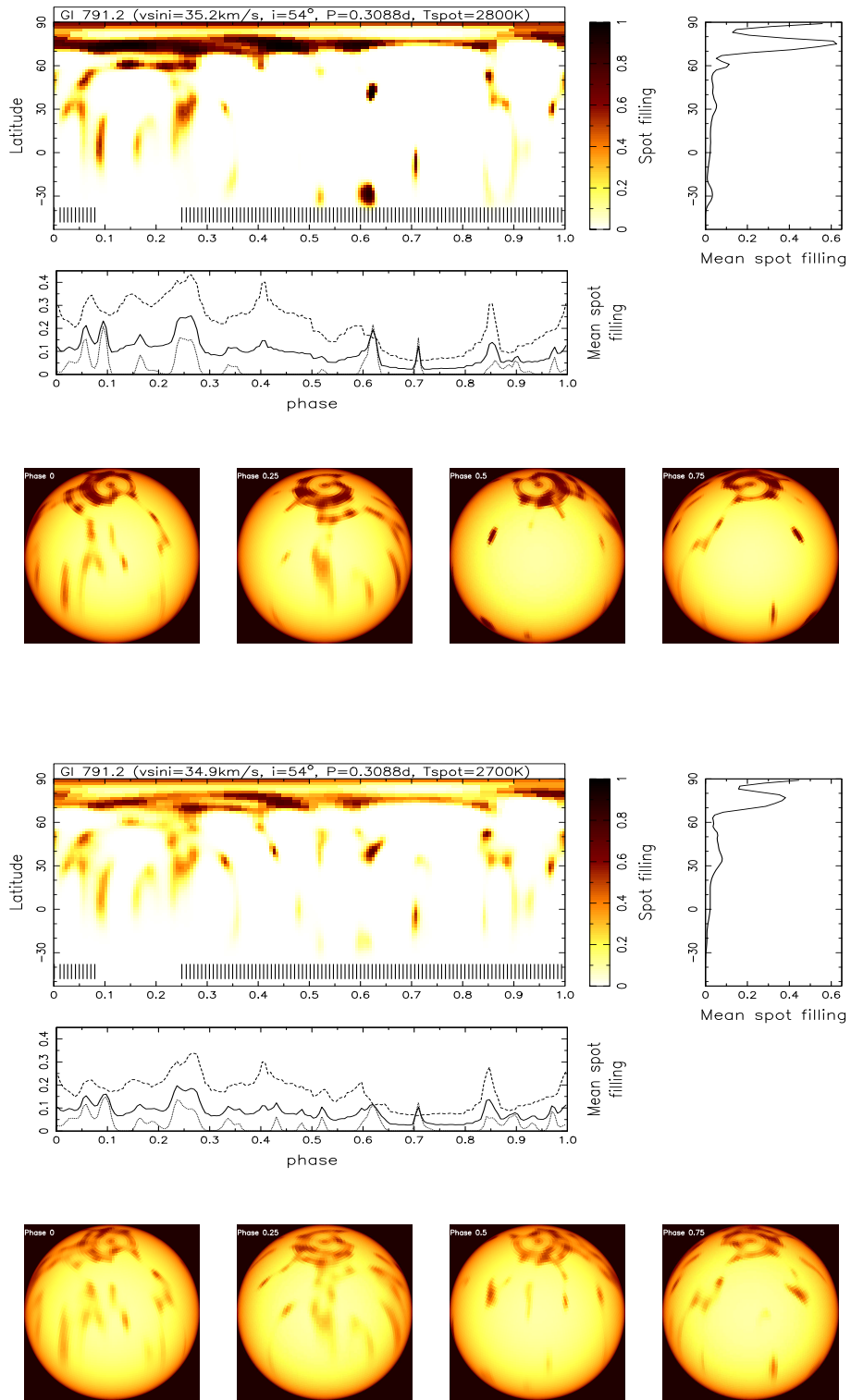
Fig. 7.— As in Figure 6 for T_{\text{spot}} = 2800 \text{ K} (top), T_{\text{spot}} = 2700 \text{ K} (bottom) with limb darkening reduced by 10% with a linear centre-to-limb scaling (bottom).
