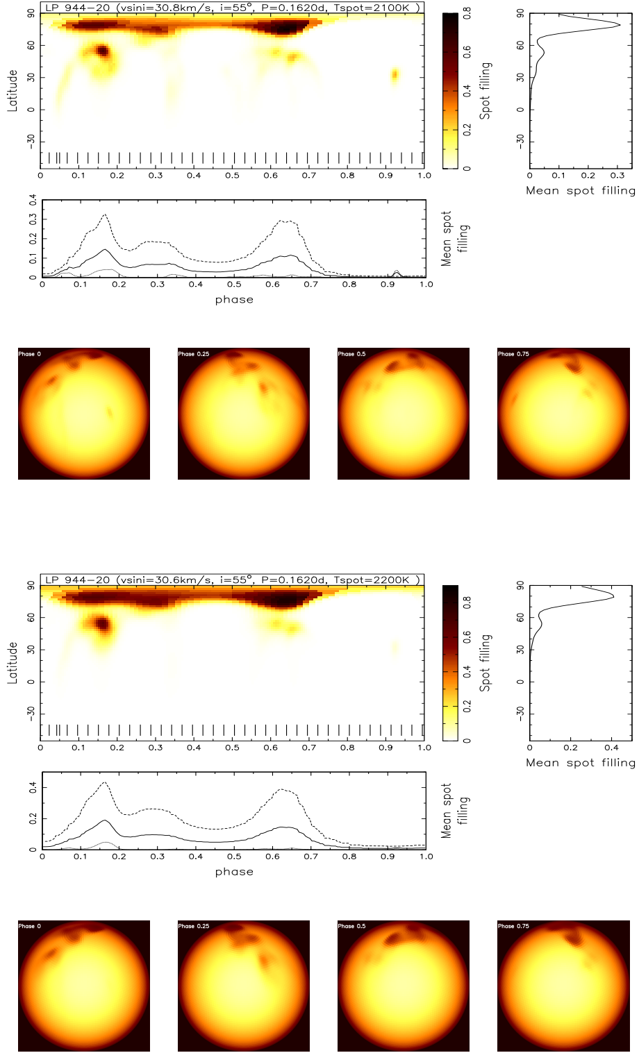
Fig. 8.— Maximum entropy regularized image reconstructions of LP 944-20 with panels as indicated in Figure 6. Images are shown for T_{\text{phot}} = 2300 K, with T_{\text{spot}} = 2100 K (upper panels) and T_{\text{spot}} = 2200 K (lower panels), with respective contrast ratios of I_{\text{spot}}(0)/I_{\text{phot}}(0) = 0.48 & 0.64.
