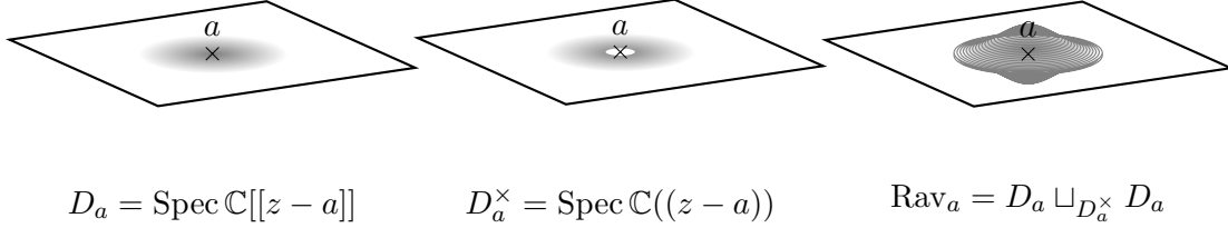
FIGURE 1. Sketch of copies of the formal disc D , the formal punctured disc D^\times , and the formal raviolo \text{Rav} associated to a point a in the complex plane.
