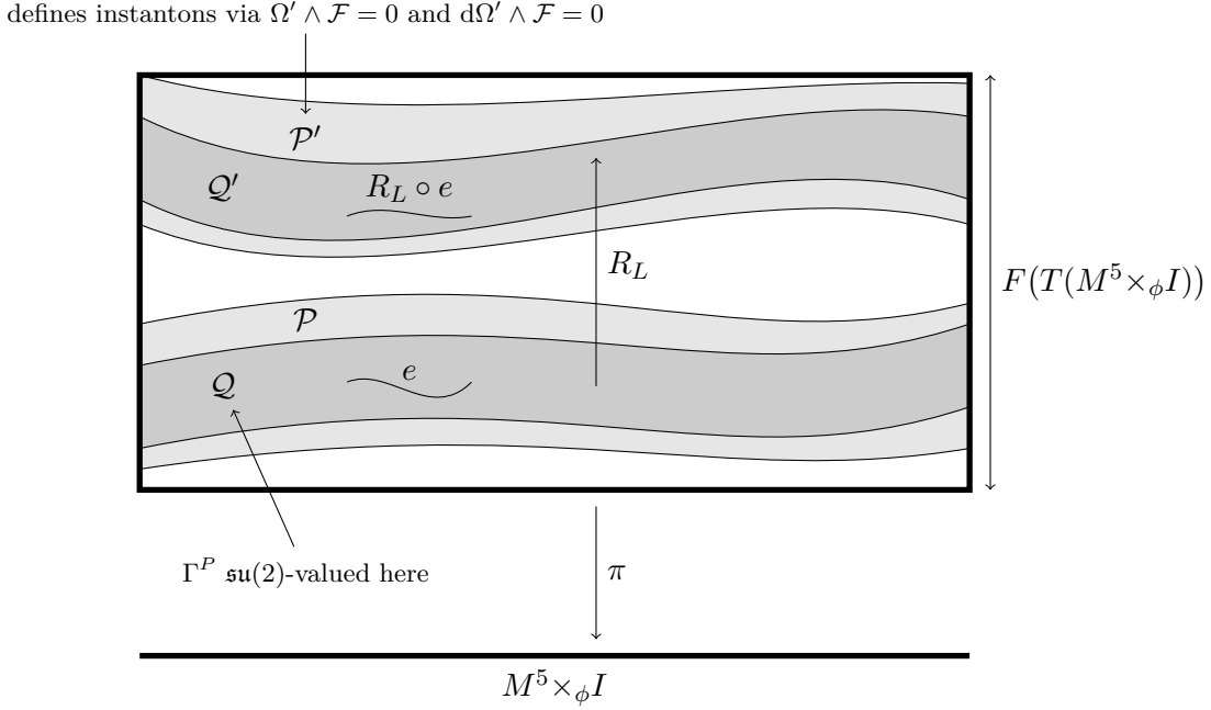
Figure 1: A schematic depiction of the different principal bundles involved in the definition of the instanton condition: \mathcal{Q} and \mathcal{P} are the SU(2) - and SU(3) -bundles, respectively, which originate from the Sasaki-Einstein structure on M^5 . The transformation L defines the principal bundles \mathcal{Q}' and \mathcal{P}' , which again are SU(2) and SU(3) -bundles, respectively. All bundles under consideration are understood as principal subbundles of the frame bundle F(T(M^5 \times_\phi I)) .
