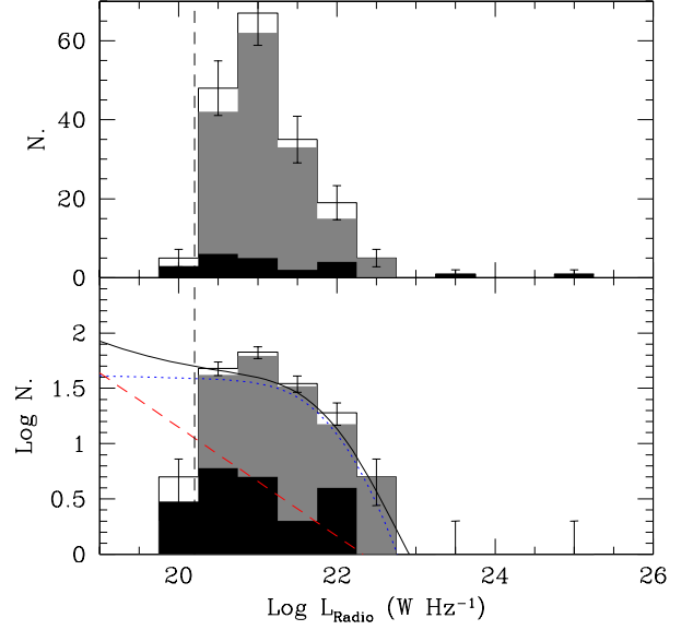
FIG. 7.— The radio continuum ( 1415 \text{ MHz} ) luminosity distribution in linear (upper panel) and logarithmic (lower panel) scales for the detected HRS galaxies (empty histogram). The black and gray histograms are for early-type (E-S0-S0a) and late-type (Sa-Sd-Im-BCD) galaxies respectively compared to the 2dF/NVSS luminosity function of Mauch & Sadler (2007) (solid line). This radio luminosity function includes both the contribution of AGN (red dashed line) and quiescent (blue dotted line) galaxies. The vertical, dashed line indicates the typical detection limit of NVSS ( 2.5 \text{ mJy} ) at the distance of 20 Mpc.
