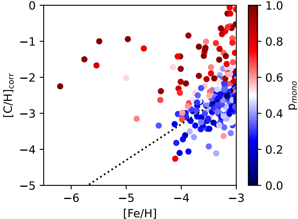
Figure 6. Carbon vs. iron abundance of EMP stars. The colour bar shows the probability for mono-enrichment. The dashed line at [C/Fe] = 0.7 should guide the eye to highlight the range of CEMP stars. There is a trend that most CEMP stars are mono-enriched.
