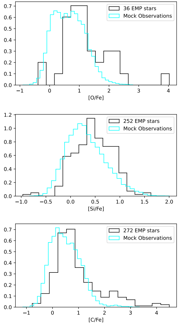
Figure 2. Comparison of the abundance distribution for the three most informative abundance ratios. While the distributions look qualitatively similar, the distribution of [O/Fe] is shifted by > 0.5 dex, which might introduce a bias in the final classification.
