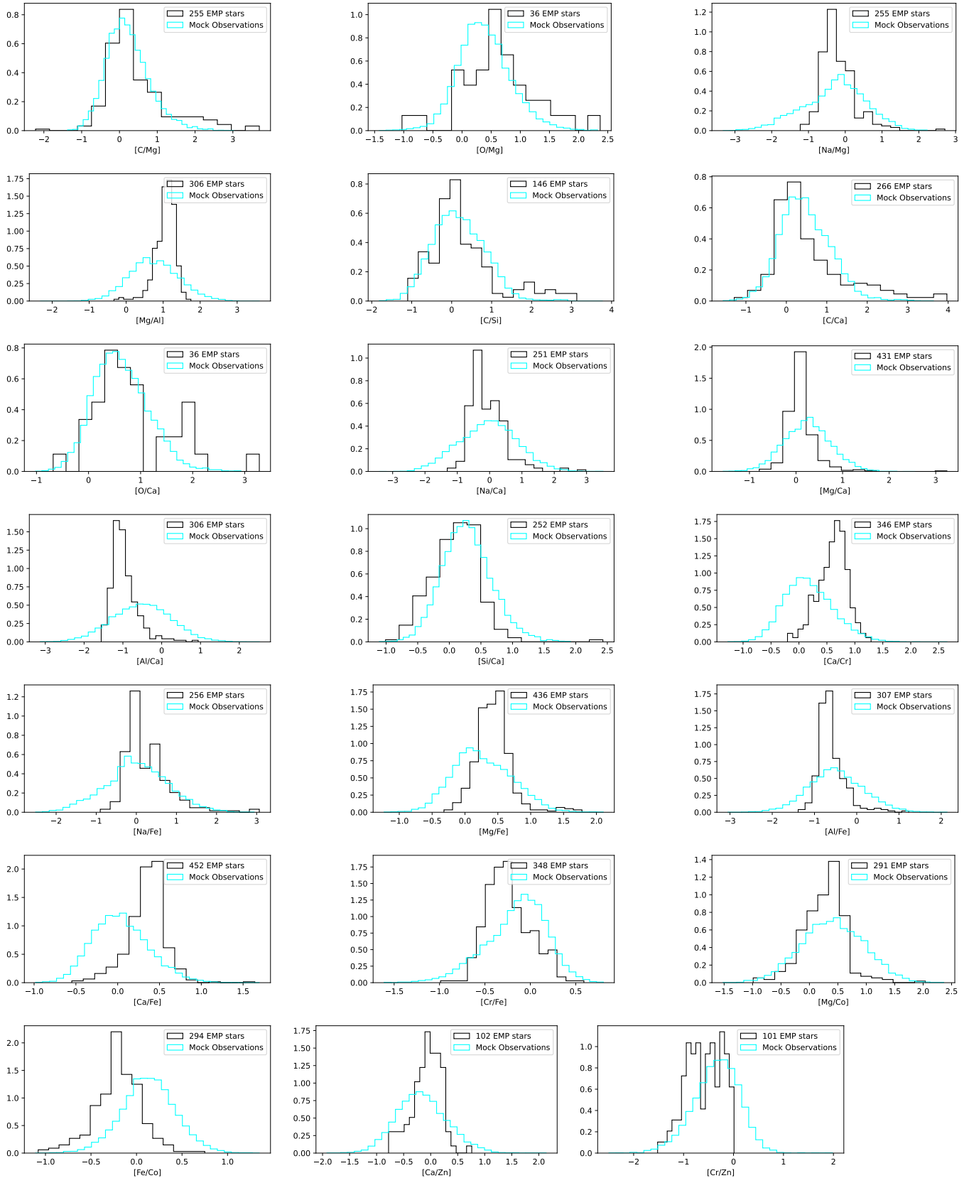
Figure 15. Same as Fig. 2, but for the remaining 21 used abundance ratios.
