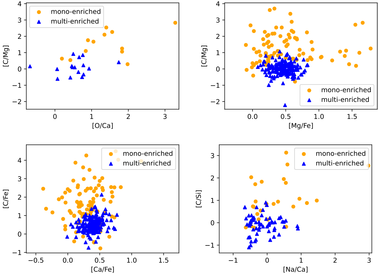
Figure 14. 2D classification maps for all EMP stars for which these abundances are available.
