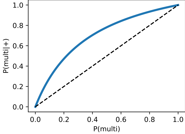
Figure 10. Probability that an EMP star that is classified as multi-enriched is actually multi-enriched as a function of the assumed multi-enriched fraction. The dashed diagonal line should guide the eye and emphasize the convex shape of the blue line.
