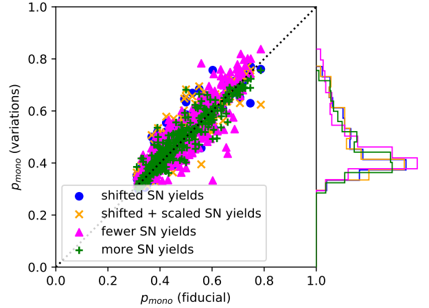
Figure 11. Predicted p_{\text{mono}} for all EMP stars. The vertical axis shows the value of four variations and the horizontal axis shows the value in the fiducial model. Most points are close to the diagonal line which illustrates that the final prediction for EMP stars is robust with respect to the exact selection of input yields. The vertical histograms on the right show the marginal distributions of the four variations.
