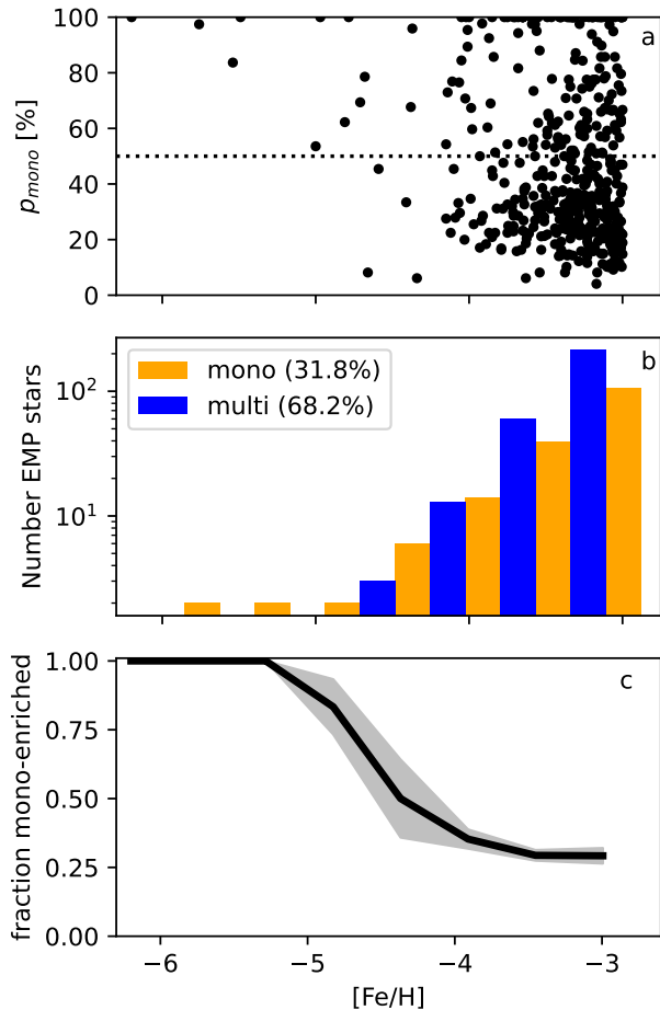
Figure 5. All panels show the results as a function of metallicity. Panel (a) shows the probability of mono-enrichment, p_{mono} , for individual EMP stars. Panel (b) shows a histogram with the absolute number of classified mono-enriched (orange) and multi-enriched (blue) EMP stars in each bin (bins are slightly offset for clarity). Panel (c) shows the fraction of mono-enriched EMP stars, and the grey contour illustrates scatter due to the bootstrap resampling of observational uncertainties.
