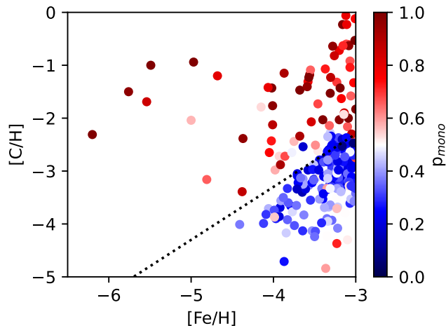
Figure 13. Same as Fig. 6 but without carbon corrections. This means that we did not use the carbon corrections for the classification, nor for the vertical axis.
