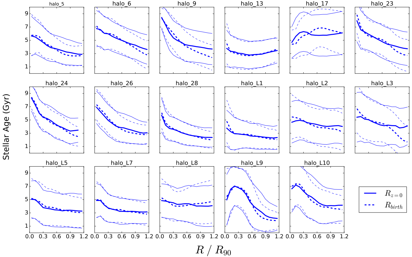
Figure 8. Mean stellar age profiles for the 17 halos in the simulation suite. The solid bold lines represent the true z = 0 profiles whereas the dashed lines are the profiles that would have been obtained if the stars were located at their birth radii instead. With the thinner lines we show the variance of stellar ages around the mean.
