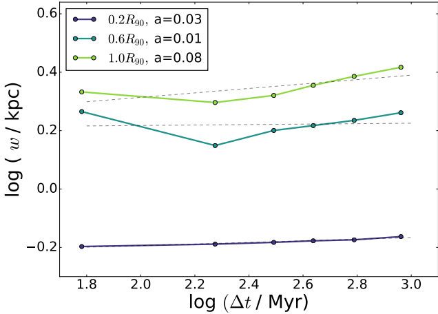
Figure 15. Logarithmic plot of the spread w against the time interval \Delta t based on the average of the combined data for all the halos. We show the trend in three different radial bins.
