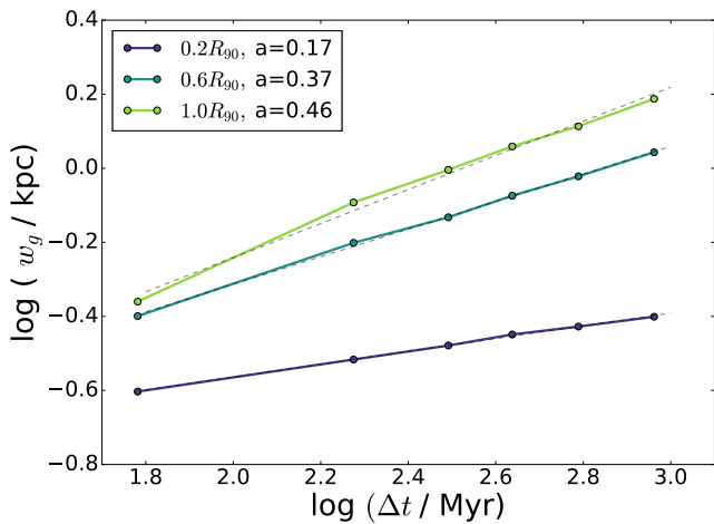
Figure 14. Logarithmic plot of the spread w_g against the time interval \Delta t based on the average of the combined data for all the halos. We show the trend in three different radial bins and observe a variation of the time interval dependence with radius, with a stronger effect being found in the outer radii.
