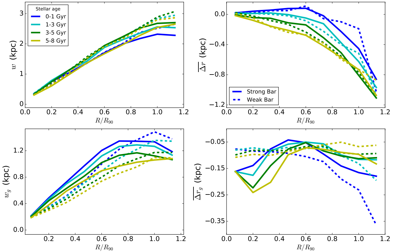
Figure 16. Similar profiles as in Fig. 13 for a fixed snapshot spacing of n + 10 , corresponding to 600-700 Myr. We split the sample between the halos that develop a strong bar, A_{2,z=0} > 0.3 , for most of their evolutionary history (solid lines) and those that have a weaker or no bar, A_{2,z=0} < 0.3 , (dashed). The different colored curves in each panel show the quantities as obtained by using only stars belonging to different age bins (legend in top left panel) selected based on their age at the initial snapshot n .
