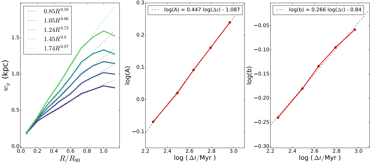
Figure 17. Left panel: Power law fits to the radial profiles of the spread w_g , referring to the spread of the \Delta R_g histograms, each curve showing a different timestep identical to Figure 13. We show the exact values for the fit in the legend. Middle and right panels: We show the logarithmic plots of the coefficient (middle) and exponent (right) of the power law against the time interval \Delta t as well as the best fit line through the data points with its functional form stated in the legend.
