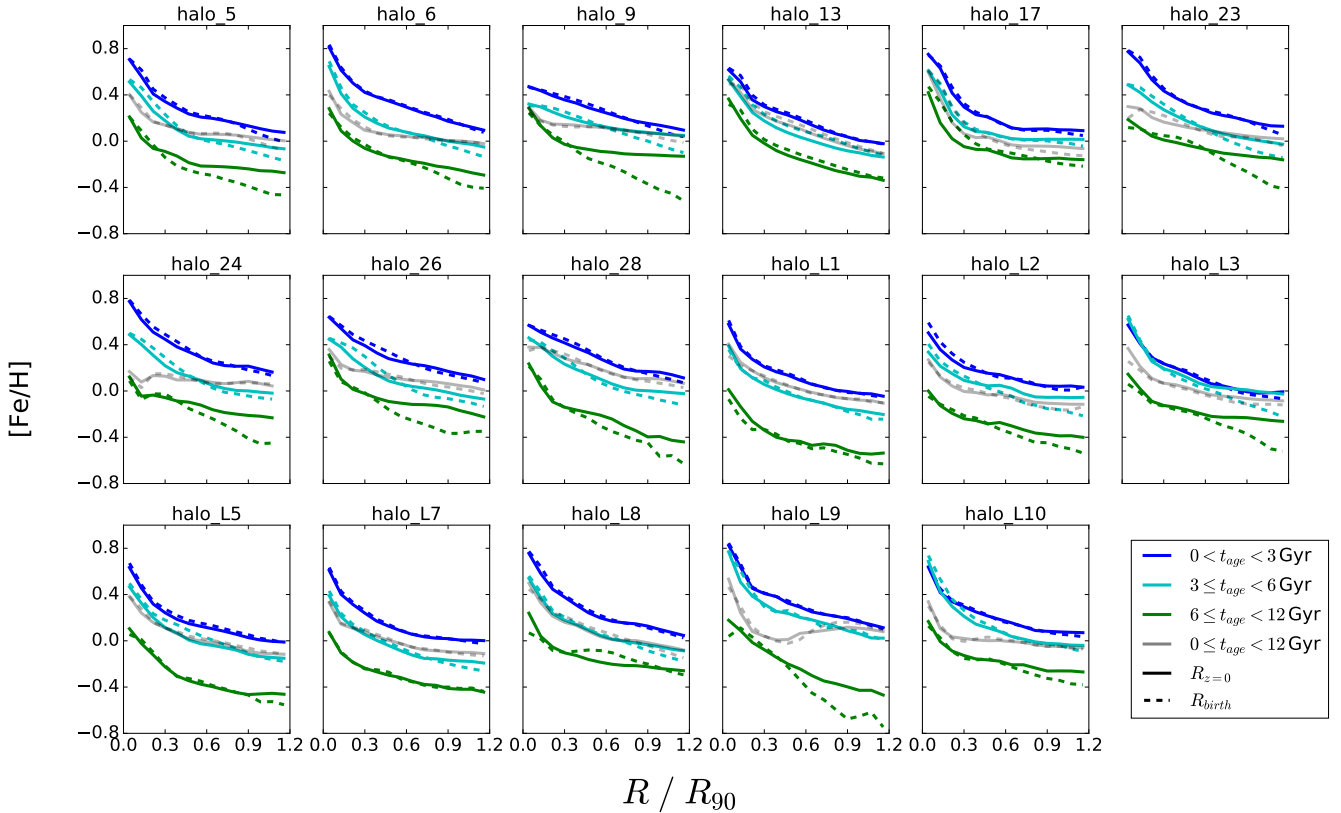
Figure 9. Radial metallicity profiles for the 17 halos in the simulation suite in three different stellar age bins. The solid lines represent the true z = 0 profiles whereas the dashed lines give the profiles that would have been obtained if the stars were located at their birth radii instead. In many cases, for the older populations, there is considerable flattening of the true metallicity profile compared to what would be produced if there was no migration. This is similar to what is presented in Minchev et al. (2013) .
