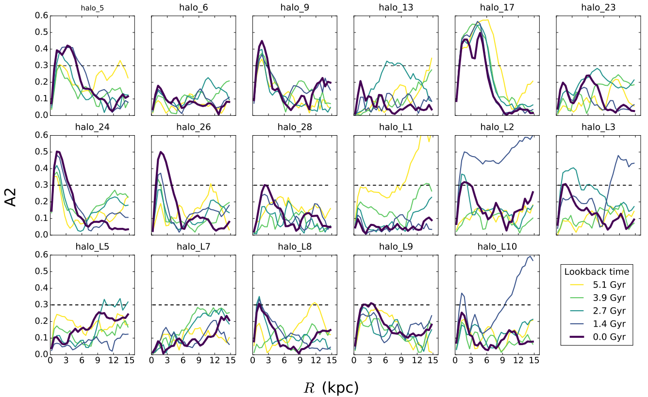
Figure 2. Measurements of the A_2 coefficient in different radii as an indicator of bar strength for our systems at several different lookback times (shown with the different color curves). The bold purple line is the measured at z = 0 . A strong bar is considered to be present when A_2 has values above 0.3 in the inner radii.
