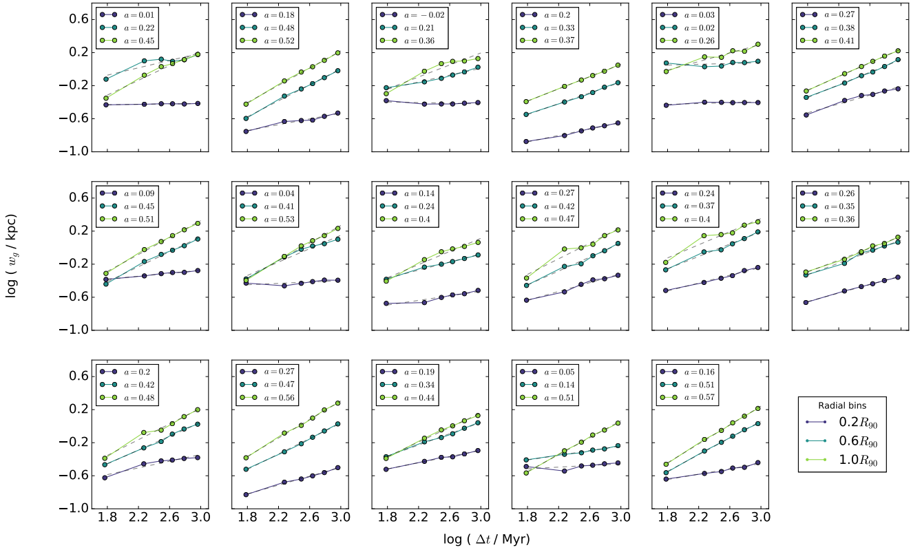
Figure A3. Logarithmic plots of the spread w_g against the time interval \Delta t for individual halos. The different curves are for different normalised radii within the disks. The slope of the best fit line is quoted in the legend in each panel. We find a variety of different values for the slopes, ranging between 0.3-0.6 in most galaxies for the two outermost rings (cyan and green).
