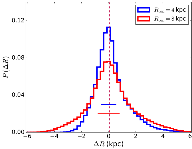
Figure A2. Example distributions of the change of the galactocentric radii for the stars selected at two given rings centred at 4 (blue) and 8 (red) kpc for ‘halo_6’. From these histograms we compute the median shift ( \overline{\Delta R} ) shown with the dashed line, and the 16-84 percentile range ( w ) shown by the horizontal lines. We observe that for the outer ring the distribution is more broadened. In both rings the shift of the median from zero is very small, and in these particular examples is slightly positive.
