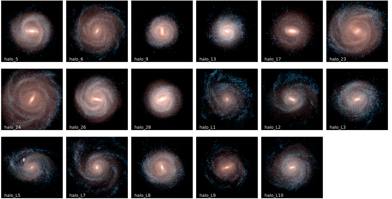
Figure 1. Stellar projections at z = 0 . The images are composites of the r , g , and i filters, and are rotated into the x - y plane of the disk. The extent of all panels is 25 \times 25 kpc.
