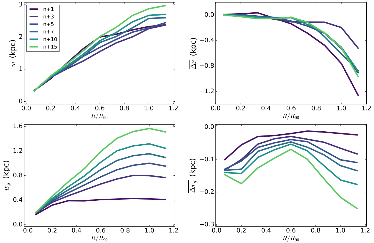
Figure 13. Mean radial profiles of the quantities that describe the distributions of \Delta r and \Delta r_g plotted in terms of the normalised ring radii. In the left panels we plot the spread of the histograms and in the right the median. The top panels are for galactocentric radii and the bottom ones for the guiding centres. Here we plot these profiles for different selections of snapshot spacings between the initial and final positions to show the evolution with \Delta t . The latter appears to be more pronounced and more clearly defined when changes in guiding centres are considered.
