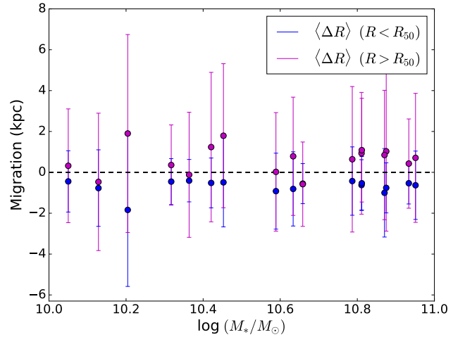
Figure 4. As Fig. 3, but for the mean migration for the stars within (blue) or outside (magenta) the half mass radius of the galaxy at redshift z = 0 . The former show on average negative values for most systems, indicating that their birth radius was in an outer region, whereas the latter have the opposite trend.
