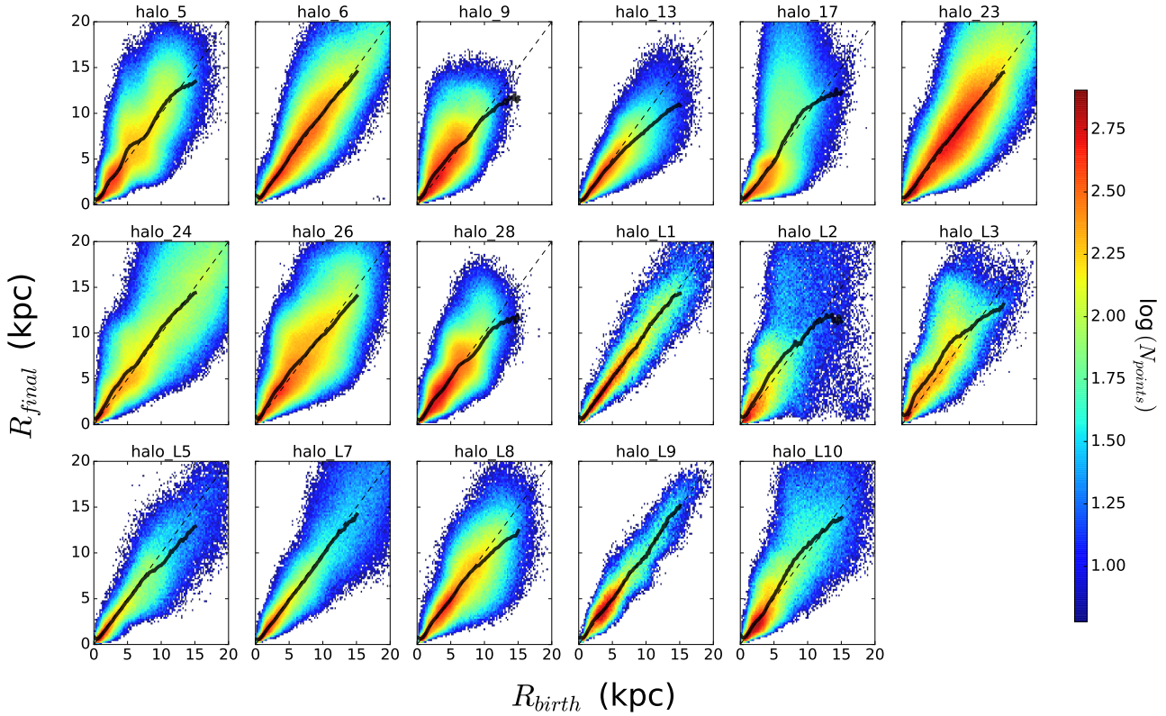
Figure 5. Birth radius versus final radius at z = 0 for all the stellar particles with circular orbits in the simulated disks. The solid line represent the median R_{\text{final}} in bins of R_{\text{birth}} and the dashed line is the one-to-one line where R_{\text{final}} = R_{\text{birth}} . Most distributions appear symmetric around the one-to-one line but there are also cases like ‘halo_17’ (5th top row) or ‘halo_9’ (3rd top row), where there are several stars above the one-to-one line, born between 5-10 kpc but having migrated outwards to 10-15 kpc.
