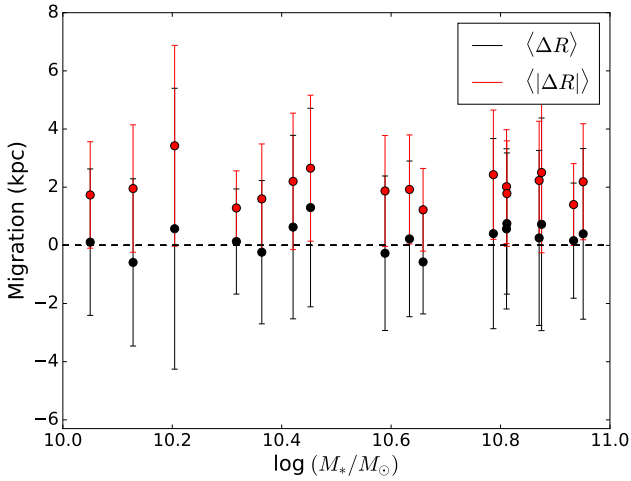
Figure 3. Mean change between the birth radius and the galactocentric radius at z = 0 , \Delta R = R_{z=0} - R_{\text{birth}} , for all disk stars and for all the systems in our sample plotted against the stellar mass at z = 0 . The black points show the average of the difference and the red the absolute value of the same quantity. The mean migration is very close to zero for all the systems.
