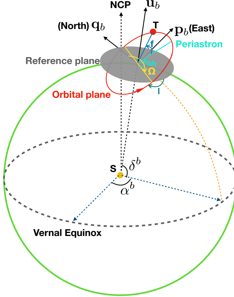
Figure 2. Illustration of the binary motion in the sky plane reference frame defined by the triad [\mathbf{p}_b \mathbf{q}_b \mathbf{u}_b] . This coordinate system is fixed at the reference epoch and does not rotate as the TSB moves with respect to the Sun. In the orbital-plane coordinate system, the x axis \mathbf{e}_x points to the periastron, the y axis \mathbf{e}_y is 90^\circ in the direction of orbital motion from \mathbf{e}_y in the orbital plane, and the z axis \mathbf{e}_z is perpendicular to the orbital plane (parallel to the angular momentum). The three axes form a right-handed Cartesian coordinate system. Here, \mathbf{q}_b points to the north while \mathbf{p}_b points to the east from the barycentric observer’s perspective. The reflex motion of the target star T is determined by the five orbital elements: semi-major axis a_T , eccentricity e , inclination I (the angle between -\mathbf{u}_b and the angular momentum), longitude of ascending node \Omega (counterclockwise angle from the north to the ascending node viewed from the observer), and argument of periastron \omega_T . The true anomaly f is needed to determine the location of the target star. For the orbit of a companion around the barycenter, the semi-major axis is a_C = \frac{m_T}{m_C} a_T where m_T and m_C are respectively the masses of the target and the companion. The argument of periastron is \omega_C = \omega_T + \pi while the other orbital elements are the same as the reflex orbit of the target star. We call the convention illustrated by this figure “astrometric convention.” This and other conventions of binary motion and the transformation between the orbital plane frame and the sky plane frame are explained in detail in Appendix A. According to equation 4, the sky plane system can be further transformed into the equatorial coordinate system defined by the Vernal Equinox and the north Celestial Pole (NCP).
