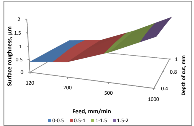
Figure 13a. Effect of DOC on surface roughness at constant spindle speed of 4000rpm (dry)
