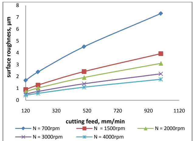
Figure 8a. Effect of cutting feed on surface roughness at constant DOC of 0.4mm (dry)
