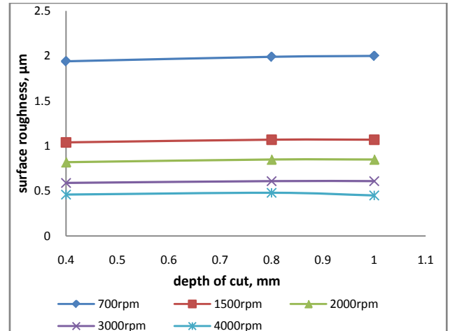
Figure 15b. Effect of DOC on surface roughness at constant cutting feed of 200mm/min (MQL)
