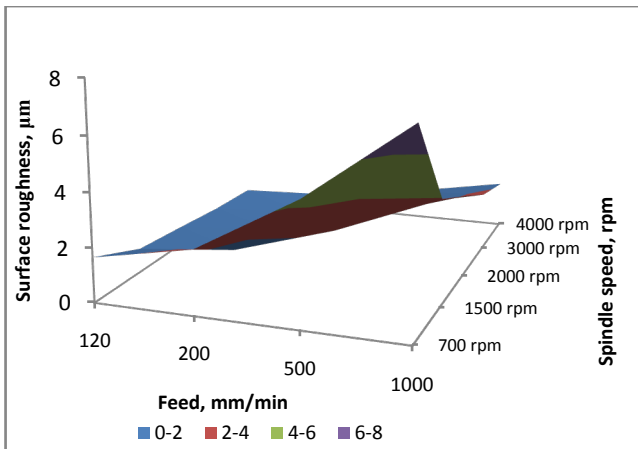
Figure 5a. Effect of spindle speed on surface roughness at constant DOC of 0.8mm (dry)
