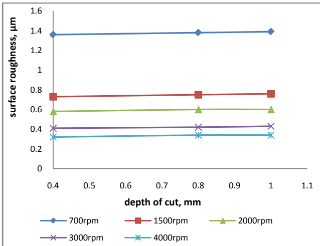
Figure 14b. Effect of DOC on surface roughness at constant cutting feed of 120mm/min (MQL)
