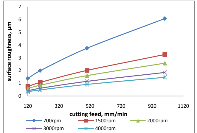
Figure 8b. Effect of cutting feed on surface roughness at constant DOC of 0.4mm (MQL)
