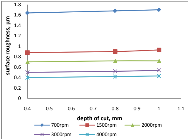
Figure 14a. Effect of DOC on surface roughness at constant cutting feed of 120mm/min (dry)
