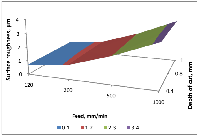
Figure 11b. Effect of DOC on surface roughness at constant spindle speed of 1500rpm (MQL)
