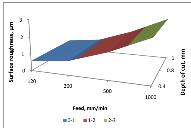
Figure 12b. Effect of DOC on surface roughness at constant spindle speed of 2000rpm (MQL)
