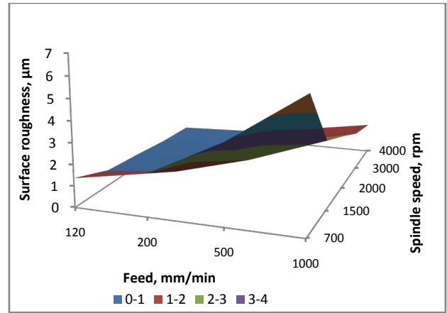
Figure 5b. Effect of spindle speed on surface roughness at constant DOC of 0.8mm (MQL)
