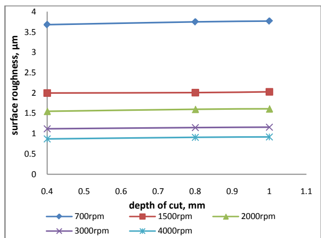
Figure 16b. Effect of DOC on surface roughness at constant cutting feed of 500mm/min (MQL)
