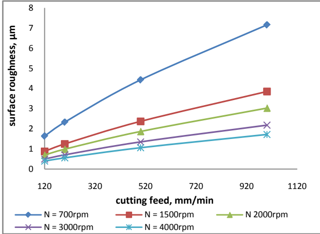
Figure 7a. Effect of cutting feed on surface roughness at constant DOC of 0.4mm (dry)
