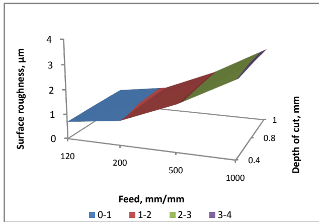
Figure 12a. Effect of DOC on surface roughness at constant spindle speed of 2000rpm (dry)
