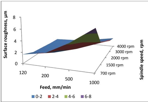
Figure 4a. Effect of spindle speed on surface roughness at constant DOC of 0.4mm (dry)
