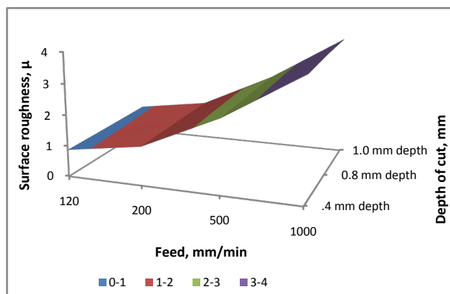
Figure 11a. Effect of DOC on surface roughness at constant spindle speed of 1500rpm (dry)
