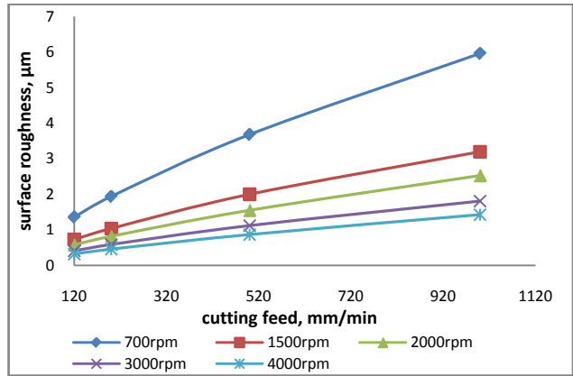
Figure 7b. Effect of cutting feed on surface roughness at constant DOC of 0.4mm (MQL)
