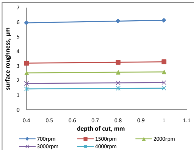
Figure 17b. Effect of DOC on surface roughness at constant cutting feed of 1000mm/min (MQL)
