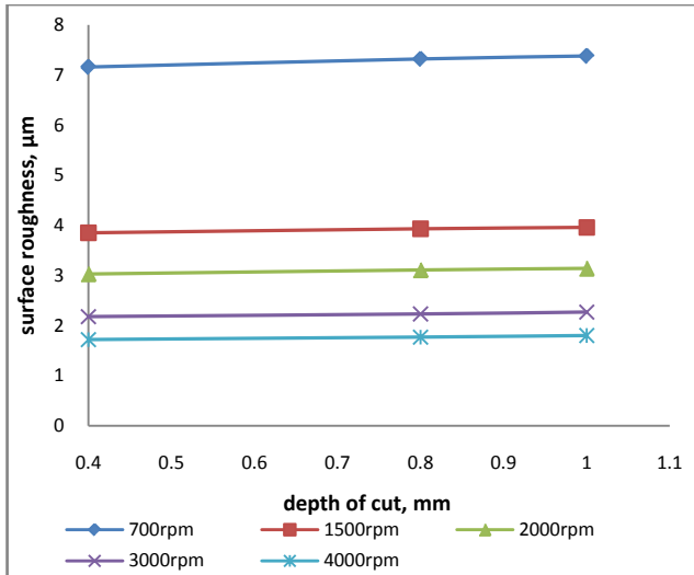
Figure 17a. Effect of DOC on surface roughness at constant cutting feed of 1000mm/min (dry)
