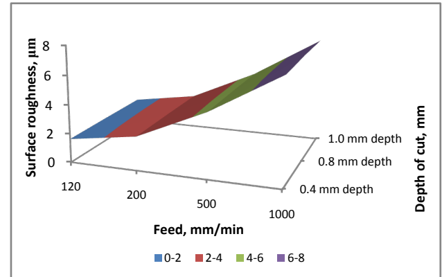
Figure 10a. Effect of DOC on surface roughness at constant spindle speed of 700rpm (dry)
