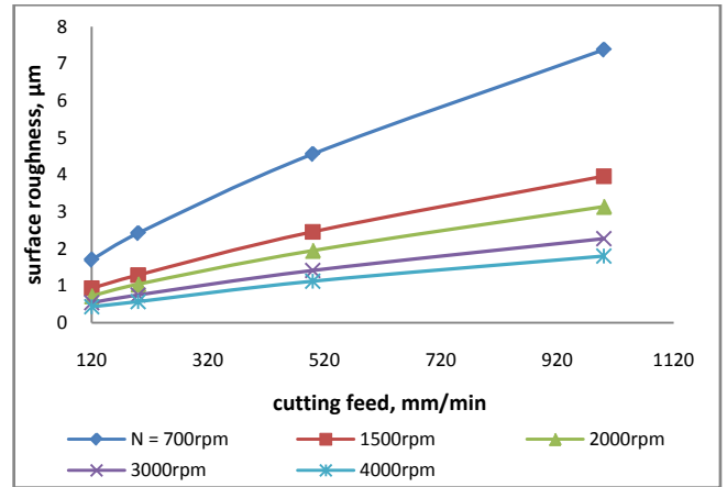
Figure 9a. Effect of cutting feed on surface roughness at constant DOC of 1.0mm (dry)
