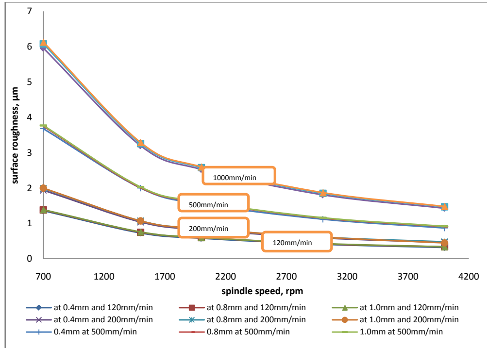
Figure 3. Effect of spindle speed on surface roughness at varying cutting feed (MQL)
