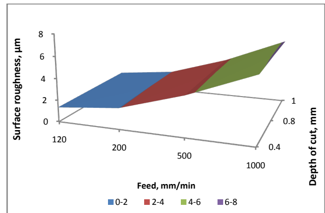
Figure 10b. Effect of DOC on surface at constant spindle speed of 700rpm (MQL)
