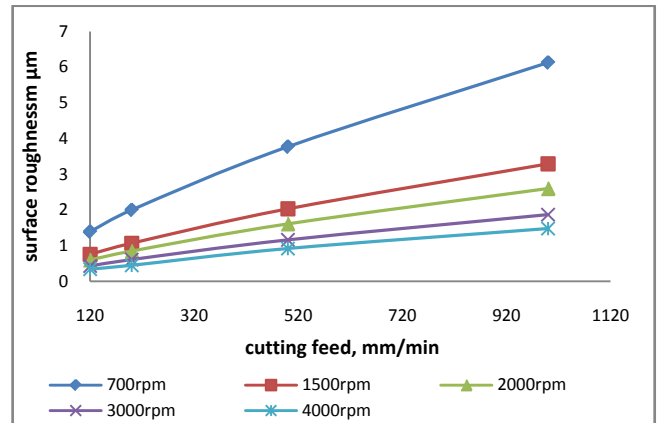
Figure 9b. Effect of cutting feed on surface roughness at constant DOC of 1.0mm (MQL)
