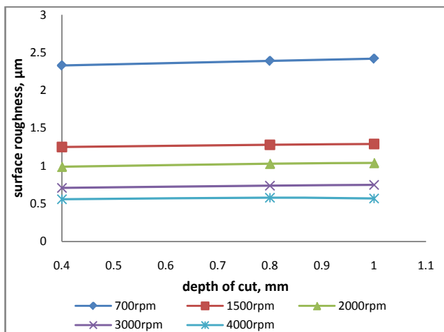
Figure 15a. Effect of DOC on surface roughness at constant cutting feed of 200mm/min (dry)
