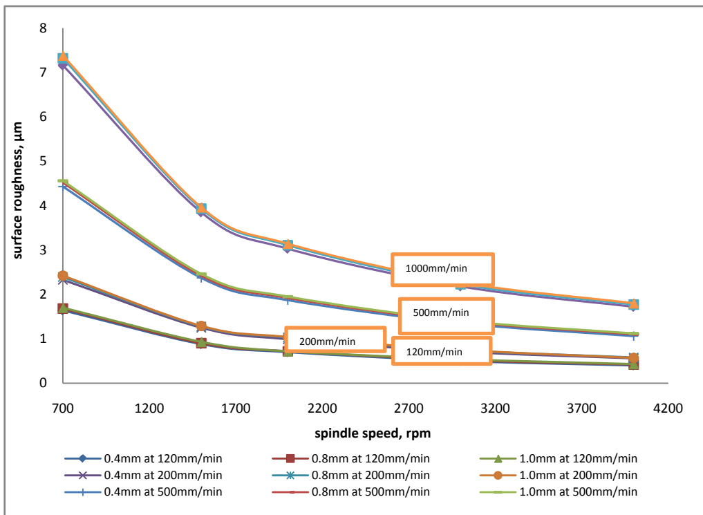
Figure 2. Effect of spindle speed on surface roughness at varying cutting feed (dry)
