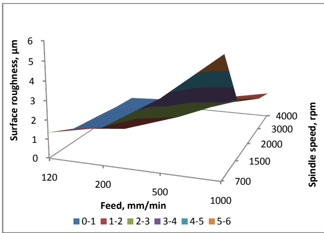
Figure 4b. Effect of spindle speed on surface roughness at constant DOC of 0.4mm (MQL)
