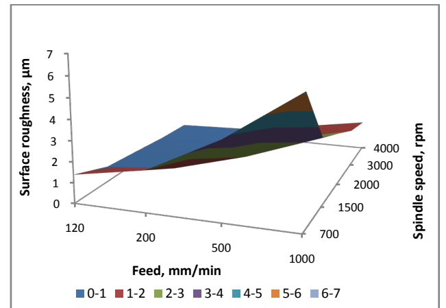
Figure 6b. Effect of spindle speed on surface roughness at constant DOC of 1.0mm (MQL)
