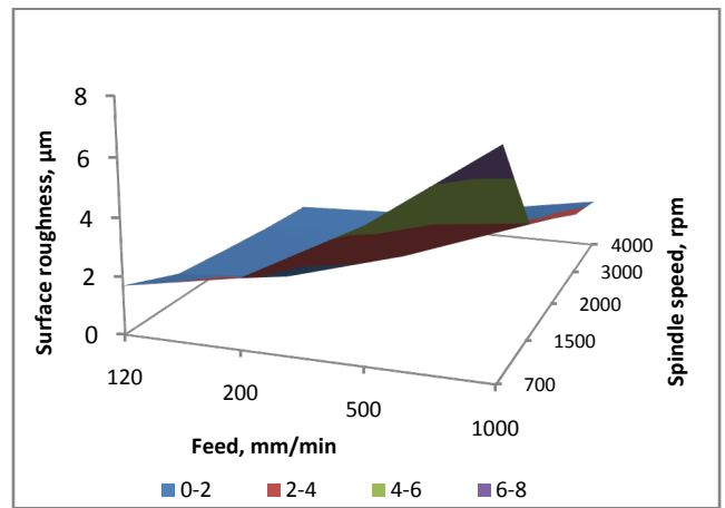
Figure 6a. Effect of spindle speed on surface roughness at constant DOC of 1.0mm (dry)
