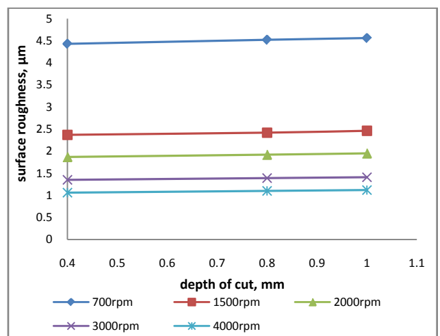
Figure 16a. Effect of DOC on surface roughness at constant cutting feed of 500mm/min (dry)
