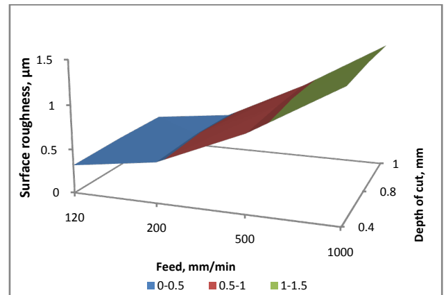
Figure 13b. Effect of DOC on surface roughness at constant spindle speed of 4000rpm (MQL)
