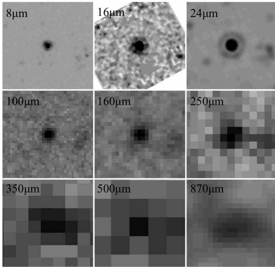
Figure 1. Postage-stamp IR images, 70 \times 70 arc-seconds, of the Spiderweb Galaxy (RA 11:40:48.60, Dec. -26:29:8.50 ; J2000) with North up and East to the left. From top left to bottom right the images are: Spitzer /8/16/24 \mu\text{m} , PACS/100 and 160 \mu\text{m} , SPIRE 250/350/500 \mu\text{m} and LABOCA/870 \mu\text{m} . The 8 and 16 \mu\text{m} band are shown for illustration only and are not used in the model fitting. Note the Airy ring is quite prominent in the Spitzer data.
