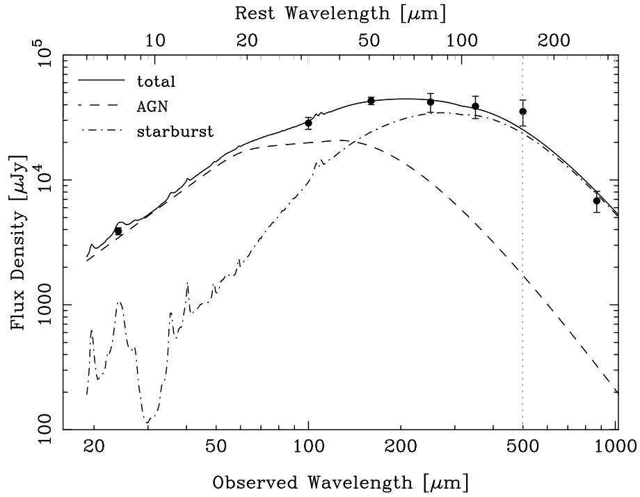
Figure 2. SED fit to the rest-frame 5–300 \mu\text{m} rest-frame photometry (black dots) of the Spiderweb Galaxy at z = 2.156 (MRC1138-262). The total model fit, and AGN and starburst components are indicated in the figure. The vertical grey dotted line represents the position of the [CII]158 \mu\text{m} line.
