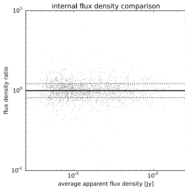
Fig. 4. Ratio of flux densities (dots) of bright, compact sources in overlapping pointings as a function of their mean apparent flux density (i.e. uncorrected for primary beam attenuation). The median and \pm 1\sigma is indicated by the full and dotted lines, respectively.
