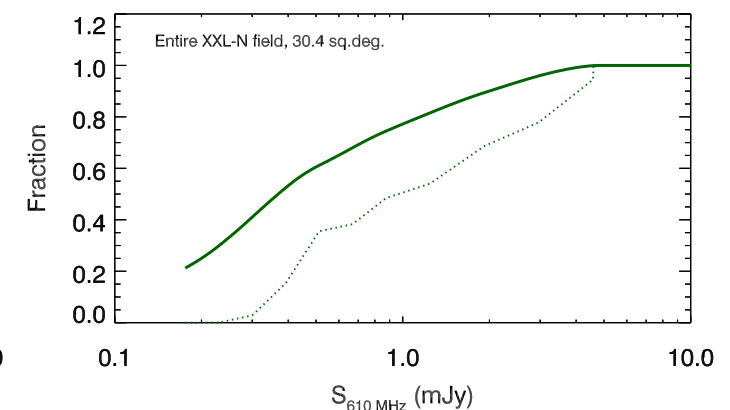
Fig. 14. Same as Fig. 14 but for the full 30.4 square degree observed GMRT-XXL-N area.
