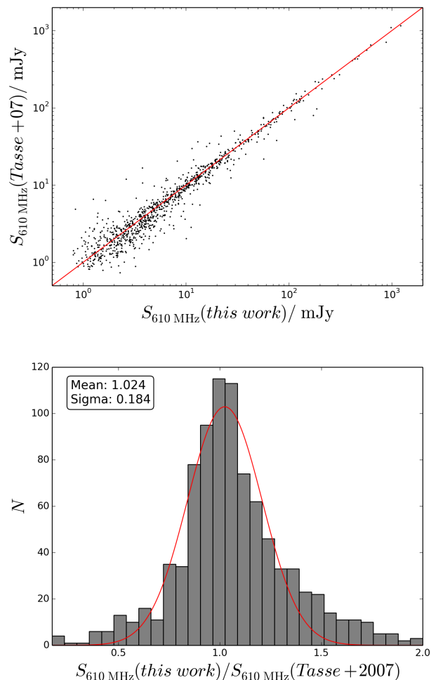
Fig. 10. Comparison within the XMM-LSS area of the XXL-N field between the flux densities obtained here (x-axis) and those extracted in the same way, but over the mosaic published by Tasse et al. (2007, y-axis; top panel). The solid line is the diagonal. The distribution of the flux ratio, with fitted Gaussian is shown in the bottom panel.
