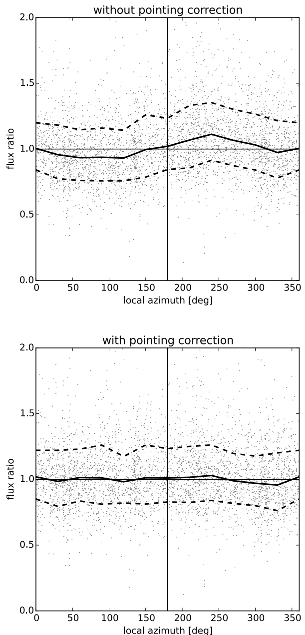
Fig. 3. Ratio of flux densities (dots) of bright, compact sources in overlapping pointings as a function of local azimuth of the source position in the first pointing before (top) and after (bottom) applying the pointing correction (see text for details). In both panels the median and \pm 1\sigma deviations are indicated by the full, and dashed lines, respectively.
