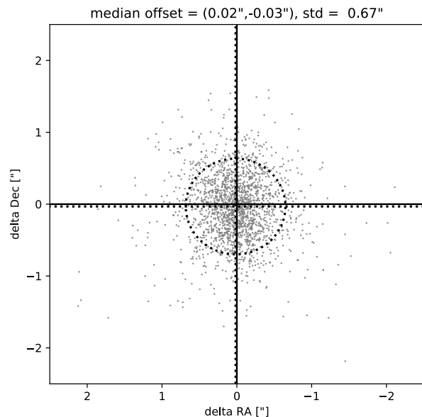
Fig. 1. Positional offsets of bright, compact sources in overlapping pointings. The median offsets in RA and Dec are indicated by the vertical and horizontal lines, respectively, while the dotted circle represents the 1\sigma deviation (also indicated at the top).
