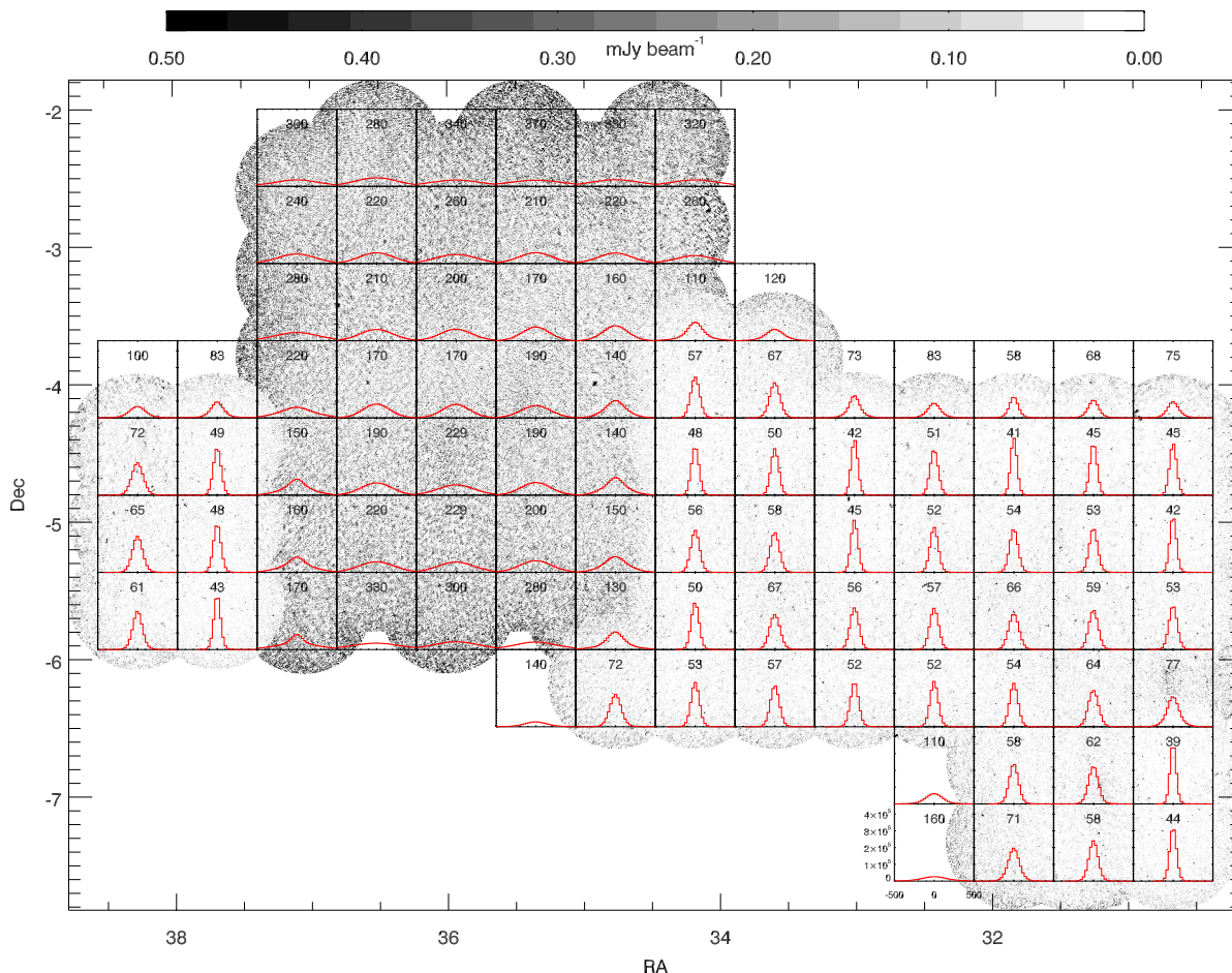
Fig. 5. Grayscale mosaic with overlaid pixel flux distributions within small areas, encompassed by the panel (the local rms in \mu\text{Jy}/\text{beam} is indicated in each panel). The x and y ranges for all the panels are indicated in the bottom left panel.
