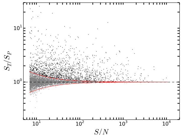
Fig. 8. Total ( S_T ) over peak ( S_P ) flux as a function of signal-to-noise ratio. The horizontal dashed line shows the S_T/S_P = 1 line. The upper curve was obtained by mirroring the lower curve (which encompasses 95% of the sources below the S_T/S_P = 1 line; see Eq. 1) over the S_T/S_P = 1 line. All sources below the upper curve are considered unresolved, while those above are considered resolved (see text for details).
