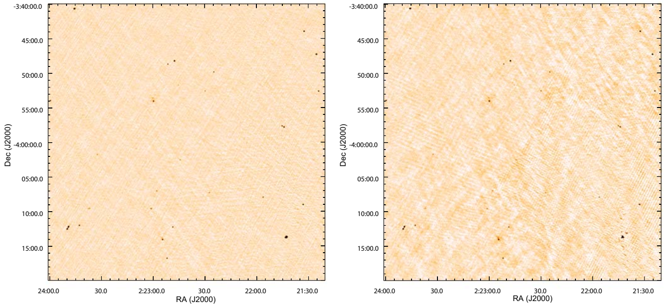
Fig. 6. Mosaiced images of the XMM-LSS area of the XXL-N field obtained by the procedure presented here (left panel) and previously published (right panel; Tasse et al. 2007), using the same colour scale.
