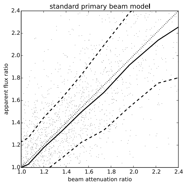
Fig. 2. Ratio of apparent flux density (i.e., not corrected for primary beam attenuation; dots) vs. ratio of the primary beam model attenuations for a sample of bright, compact sources in overlapping pointings. The median and \pm 1\sigma offsets are indicated by the full and dashed lines, respectively. The one-to-one line is represented by the dotted line.
