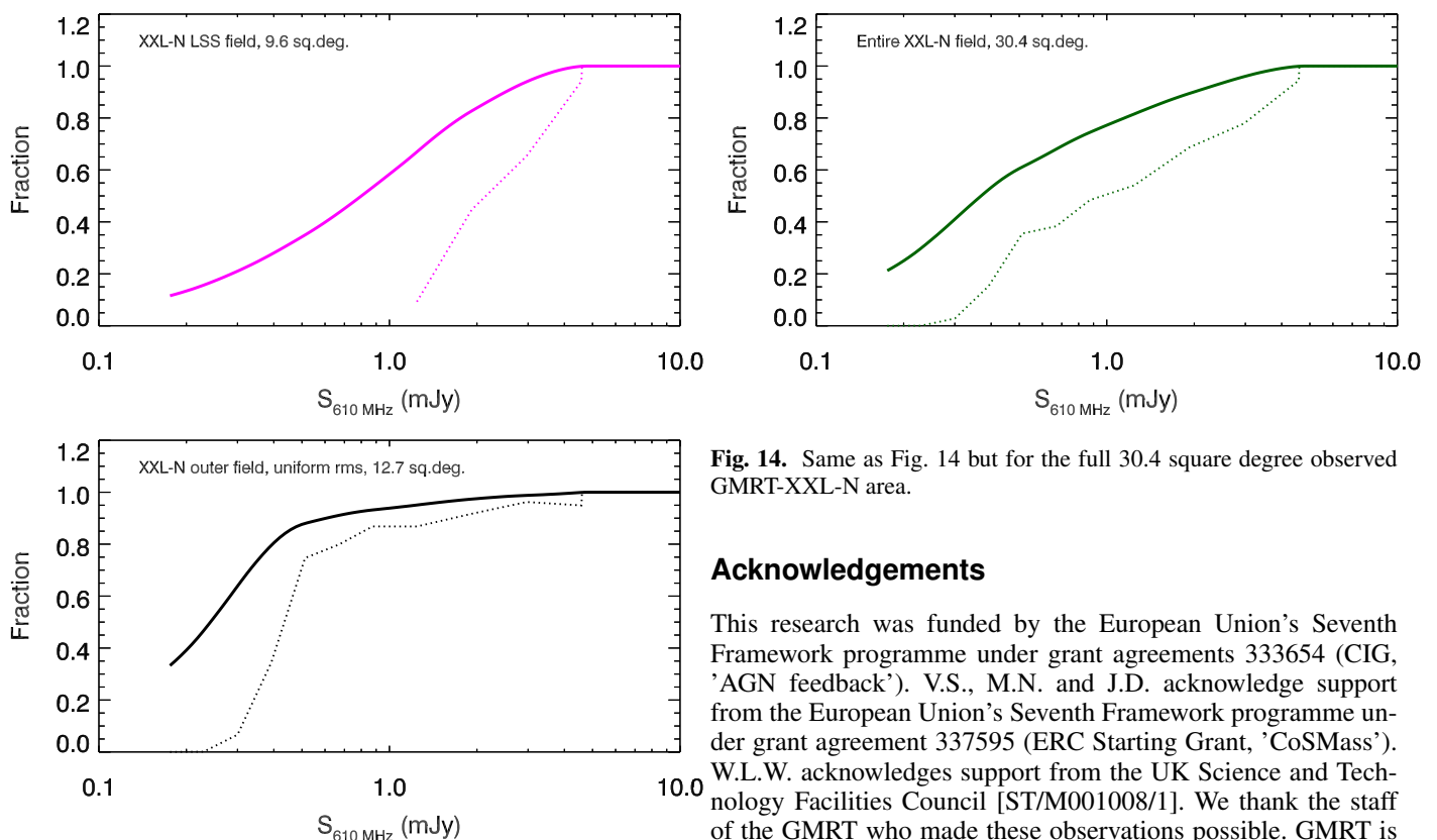
Fig. 13. Detection fraction as a function of 610 MHz flux density relative to the VLA-COSMOS 3 GHz Large Project (dashed line) for the inner area (9.6 square degrees, coincident with the XMM-LSS field; left panel) and outer area (12.66 square degree) areas. Also shown is the completeness (i.e. the detection fraction in a given bin and that above the given flux bin lower limit) as a function of flux density (full line).
